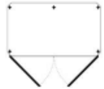
One pair center-closing doors for double-wide bays (with no center post)
